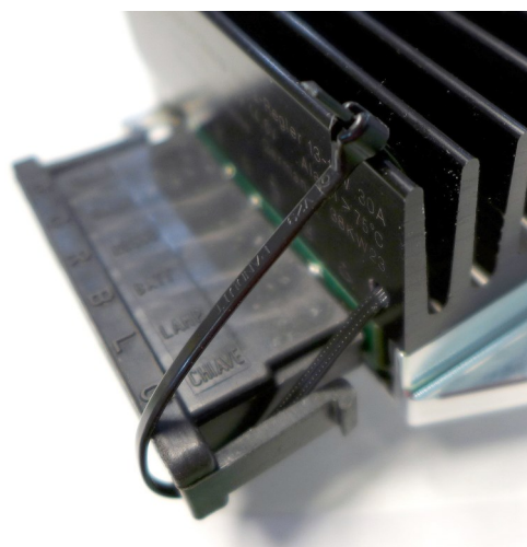
Pull secure of the combination plug with a cable tie
