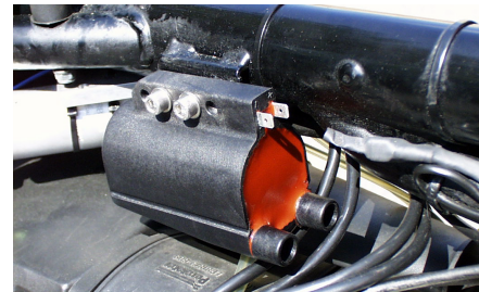
PowerCoil on the /5 frame The ignition-box can be mounted on the other side
