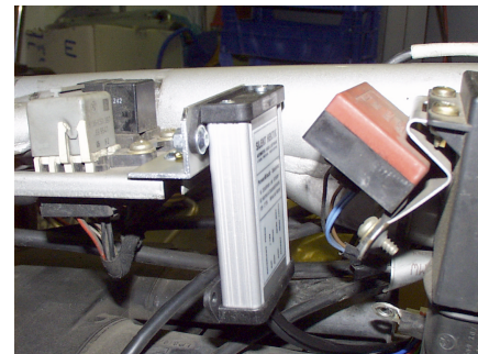
The distance from the box to coils should be min. 10cm
