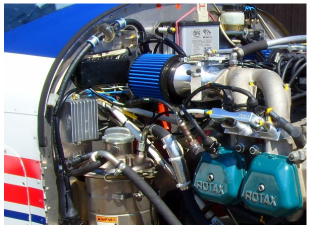
Installation in the front with good cooling by airflow and max. 70cm cables to the battery
